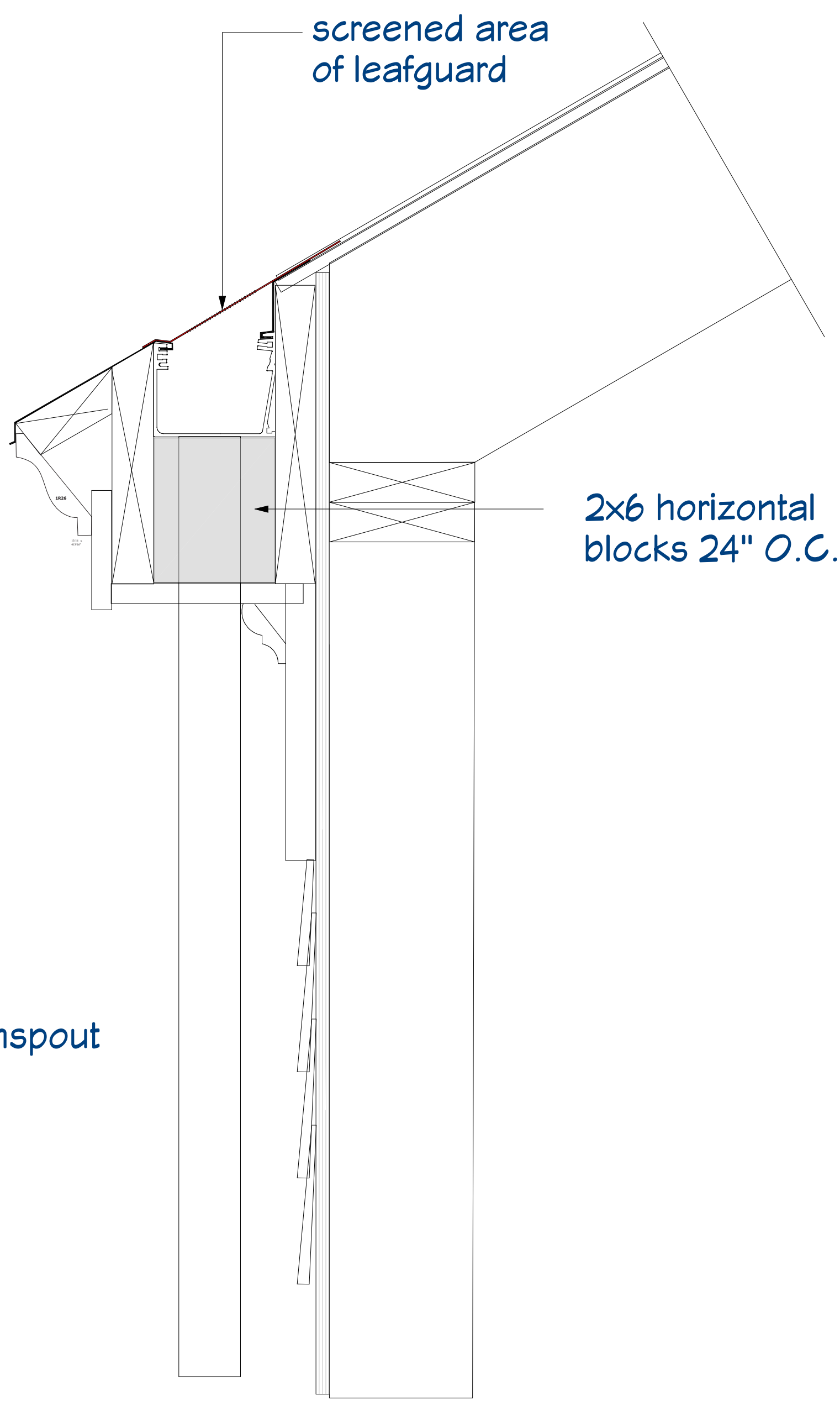
SECTION B
