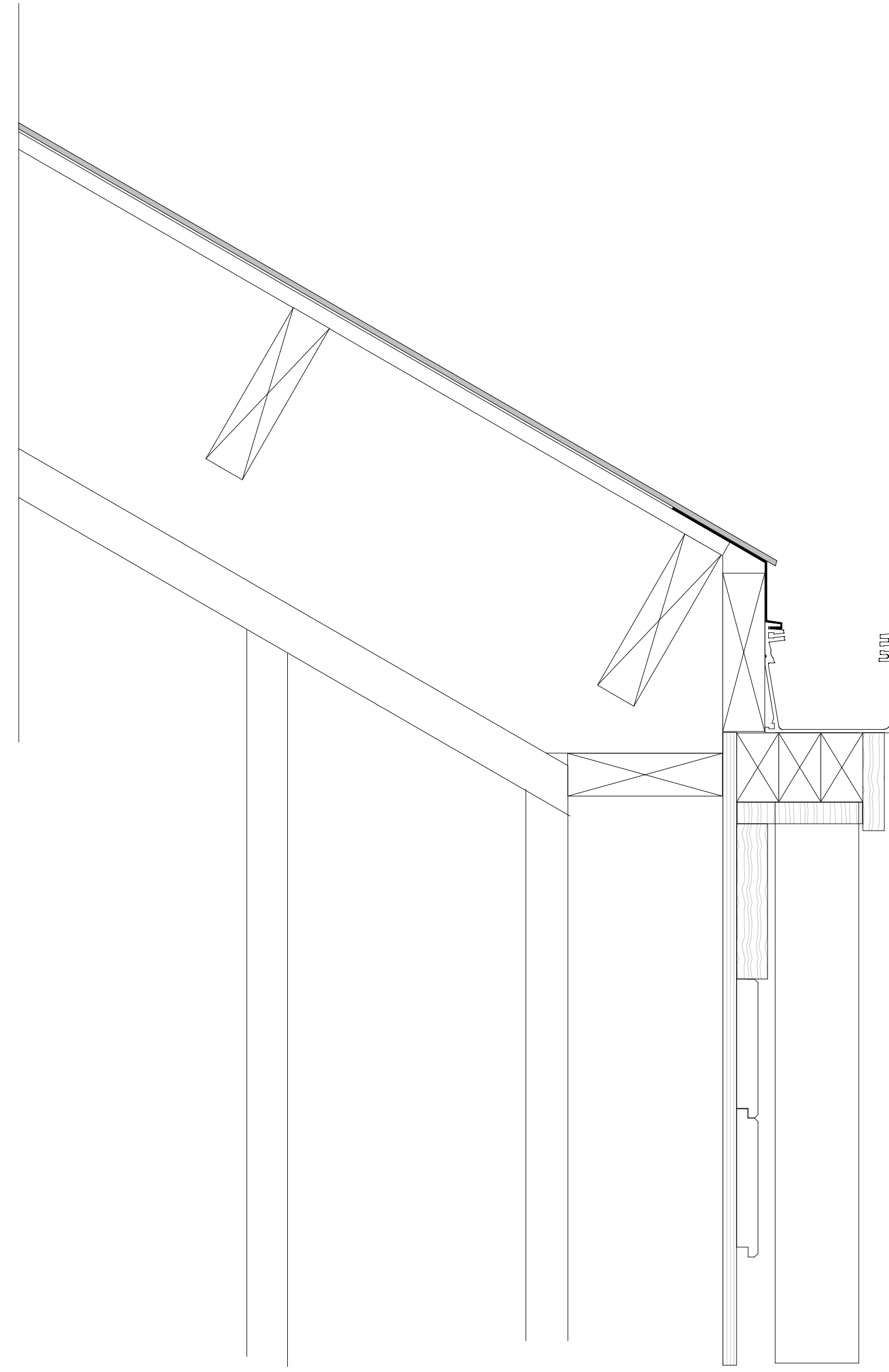
SECTION
